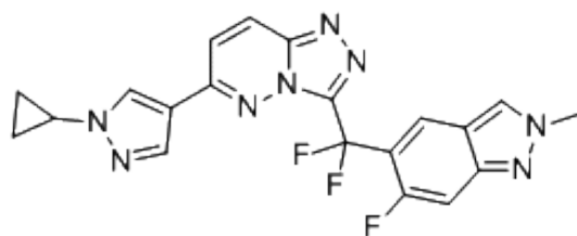
PC-3573201, DMSO-d 6
